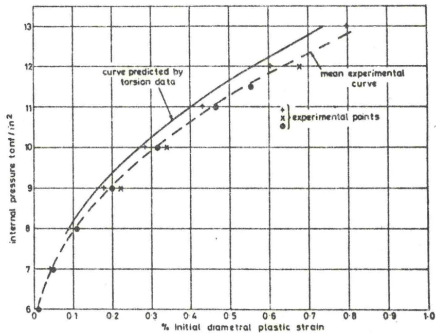
FIG. 14 COMPARISON OF PREDICTED AND EXPERIMENTAL INITIAL PRESSURE-EXPANSION CURVES (0.18 PERCENT CARBON STEEL AT 400°C)
