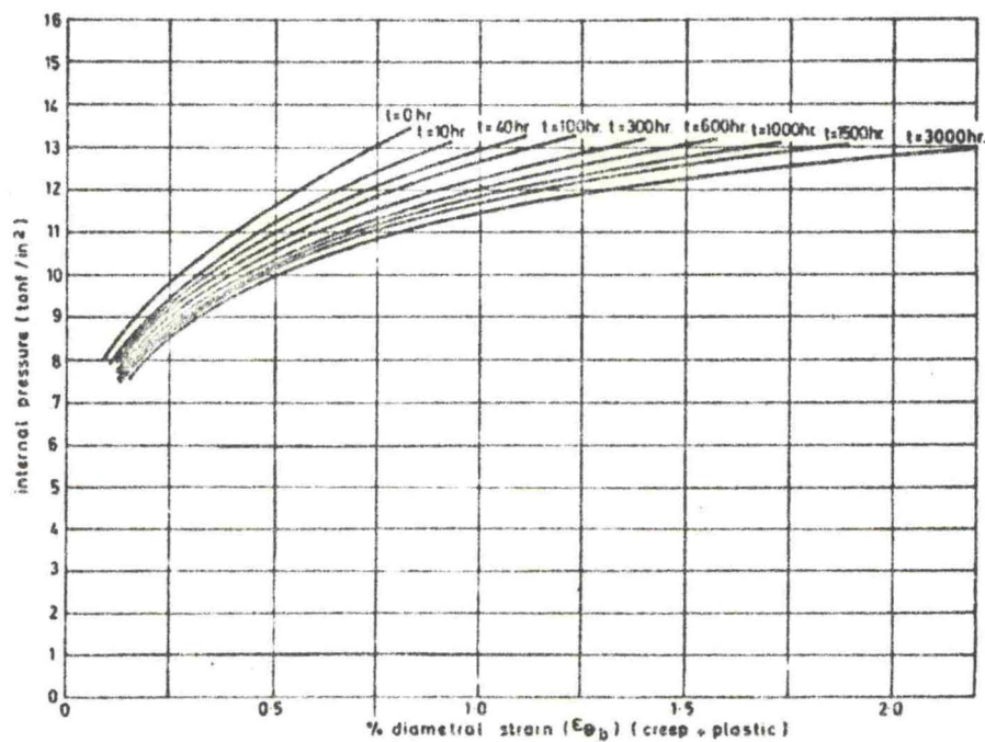
FIG. 15 ISOCHRONOUS PRESSURE-EXPANSION CURVES PREDICTED BY TORSION CREEP DATA (0.18 PERCENT CARBON STEEL AT 400°C)
